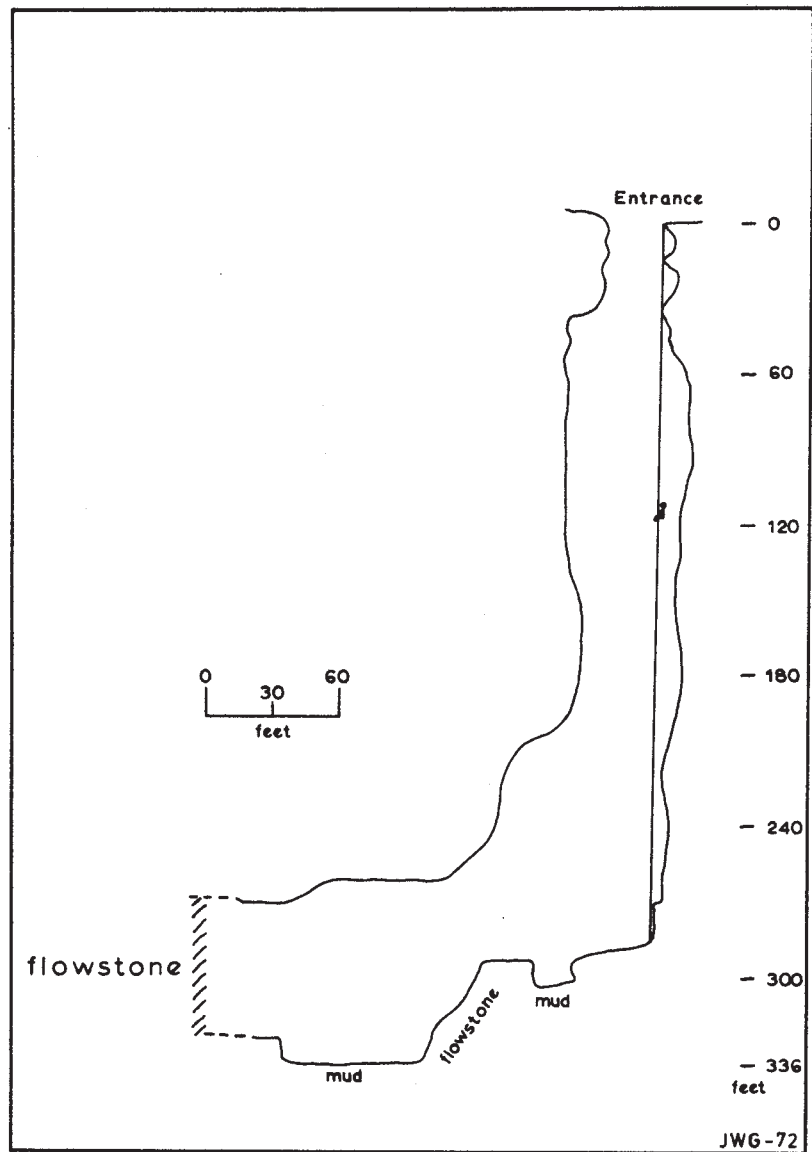
Fig. 10. Generalized cross-section, looking approximately southwest, of Site No. 15, Sótano de Meco, showing rigging point and position within shaft during rappel.
