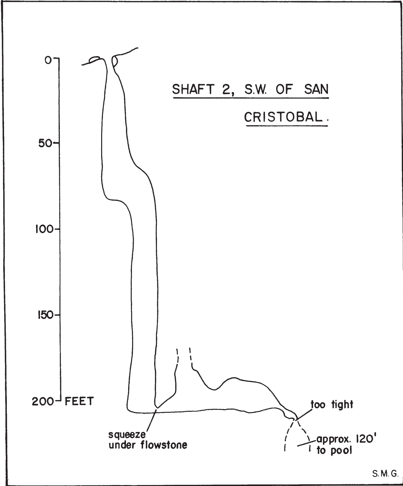
Shaft 2 Campo Grande, Mpo. Chilóh Chiapas Canadian Caver, v. 7, no. 1, p. 40, 1975
