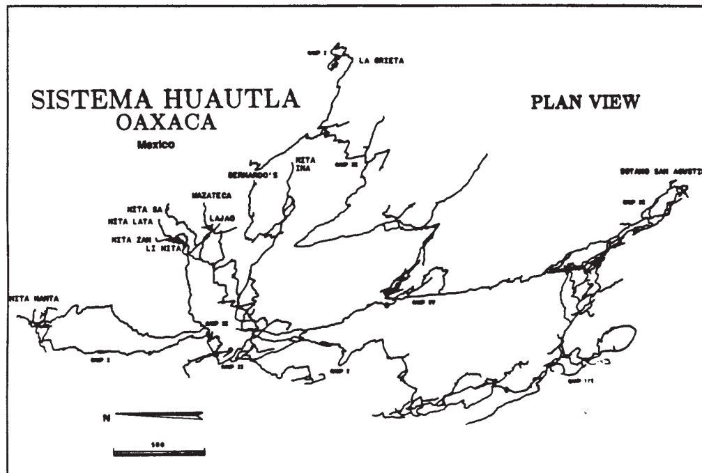
Figure 1.2c: Plan view of Sistema Huautla prior to the 1994 San Agustín Expedition
