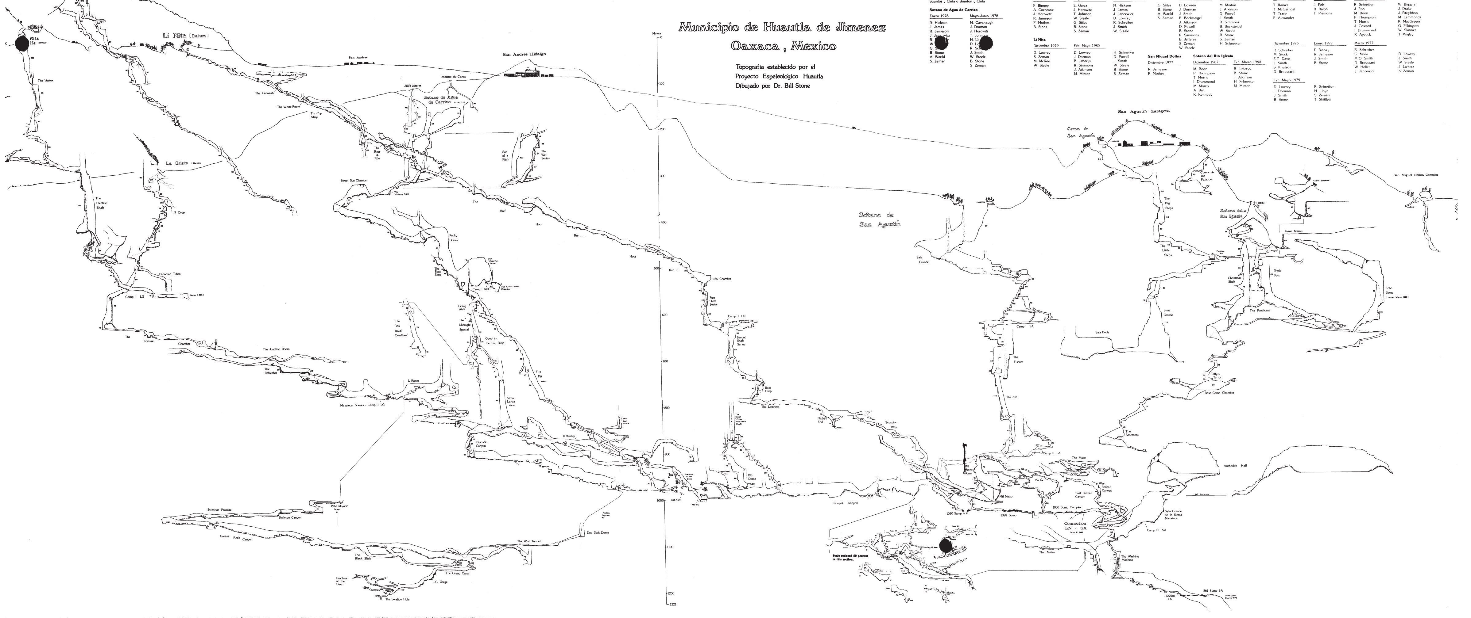
Sistema Huautla area caves Mpo. Huautla de Jiménez Oaxaca NSS News, June 1983, p. 176
