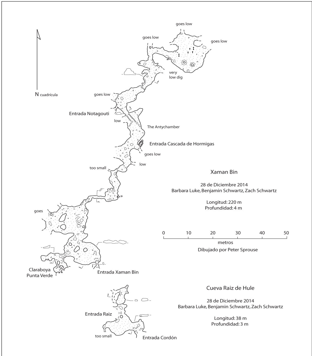
Xaman Bin, Cueva Raiz de Hule Paamul Quintana Roo AMCS Activities Newsletter 38, p. 112, 2015
